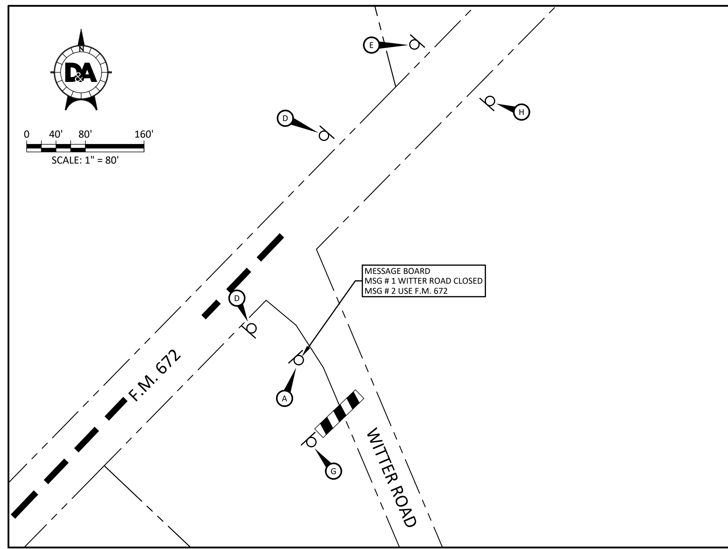
INTERSECTION "B" SCALE: 1" = 80'
