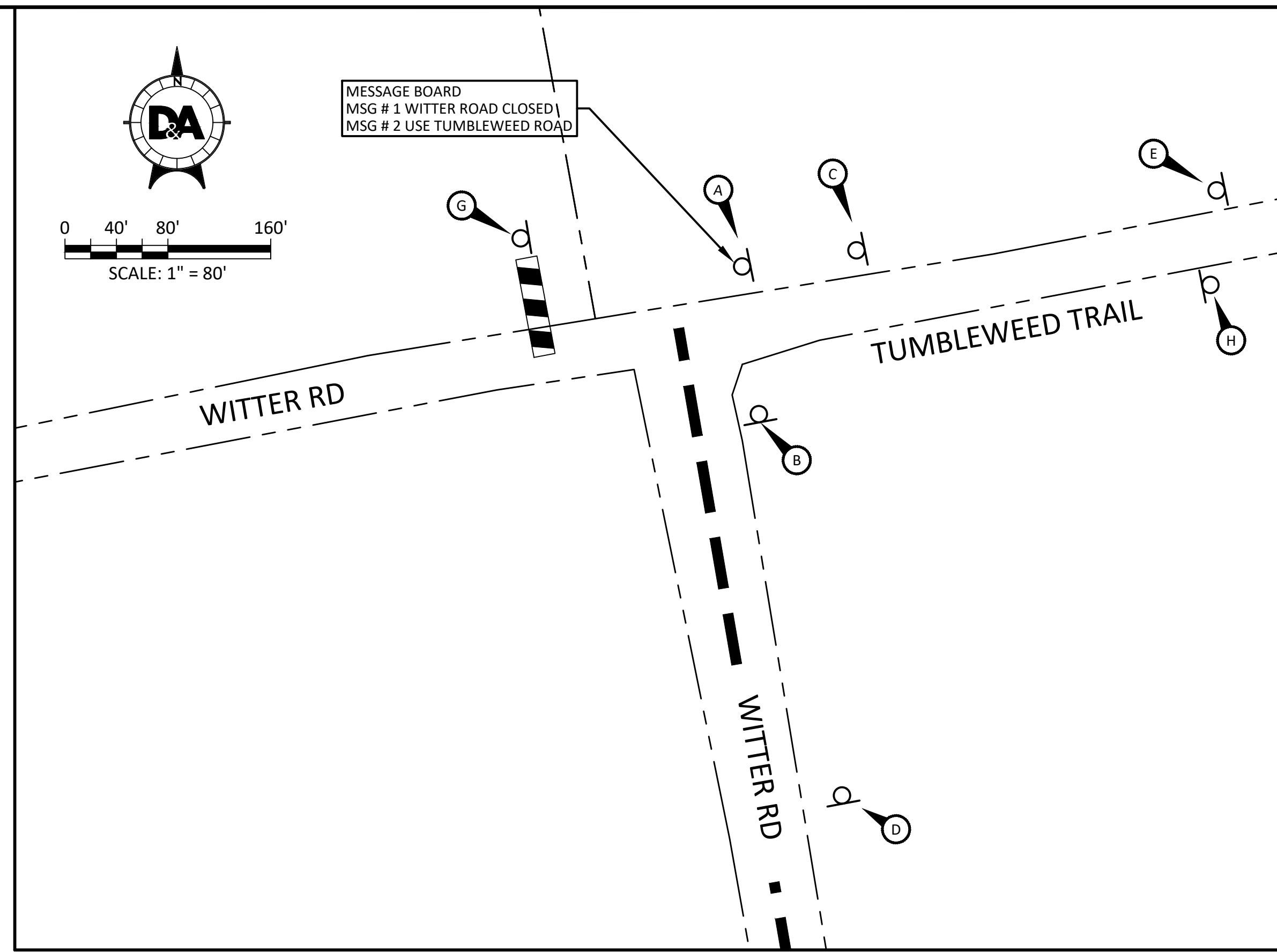
INTERSECTION "A" SCALE: 1" = 80'
